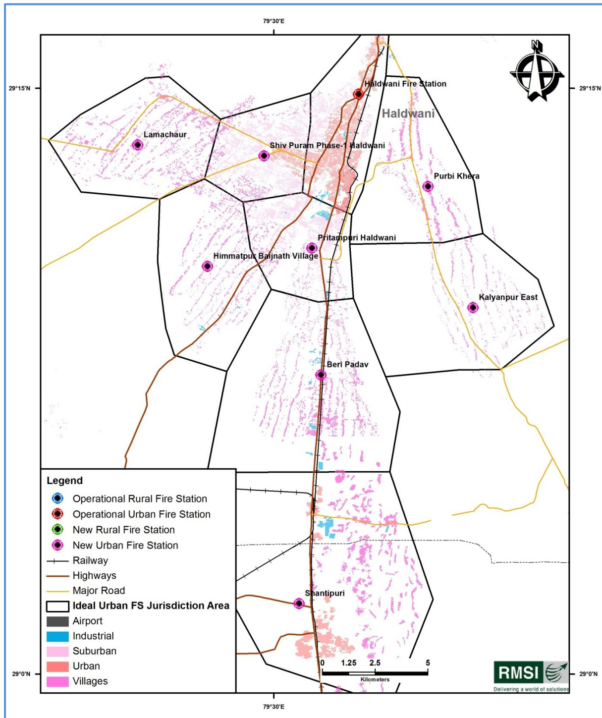
Figure 17-10: Fire Stations gap analysis for Haldwani urban areas
