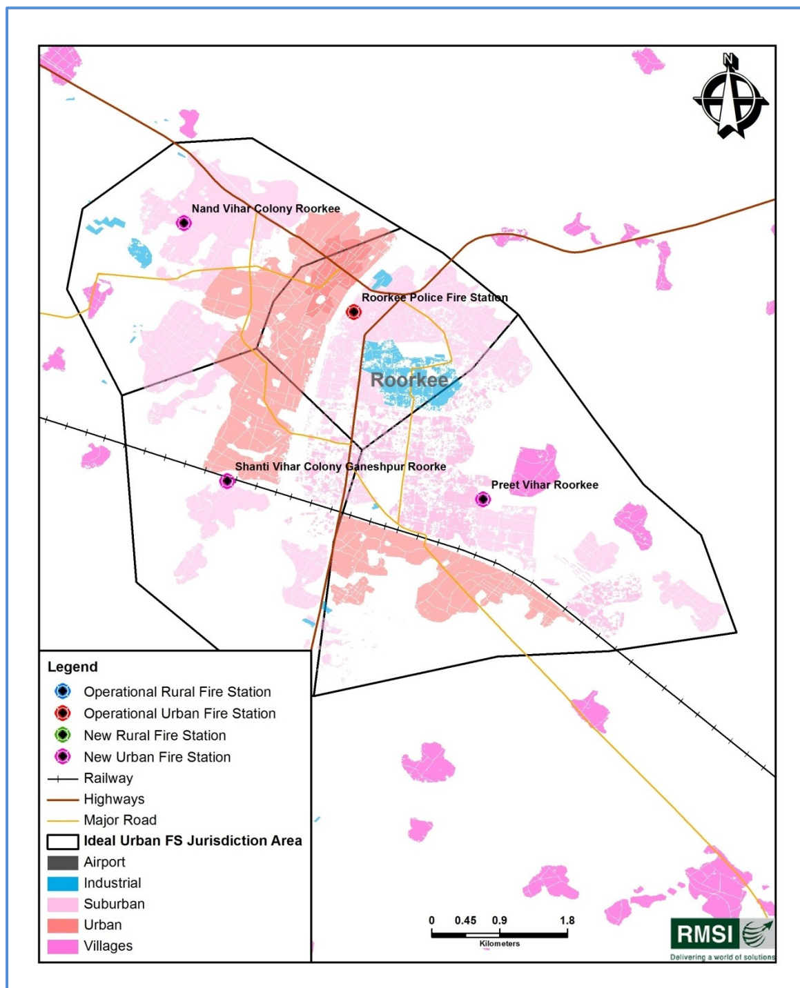
Figure 17-8: Fire Stations gap analysis for Roorkee urban areas
