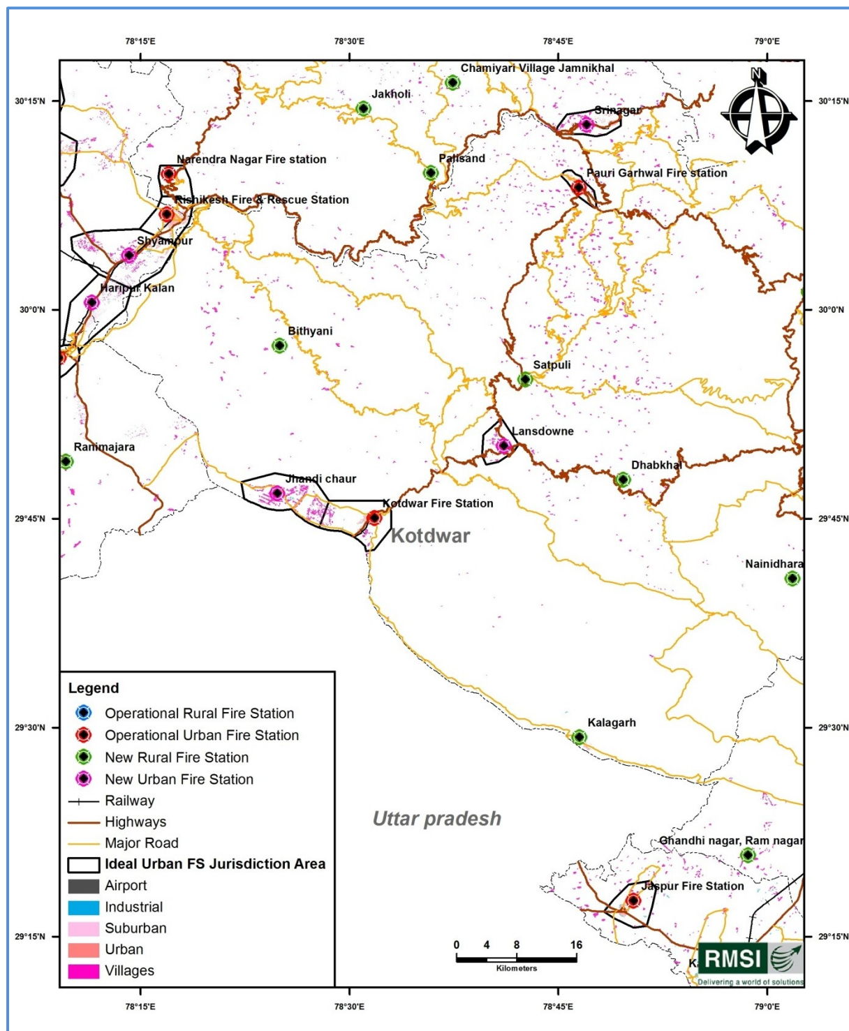
Figure 17-17: Fire Stations gap analysis for Kotdwar rural areas
