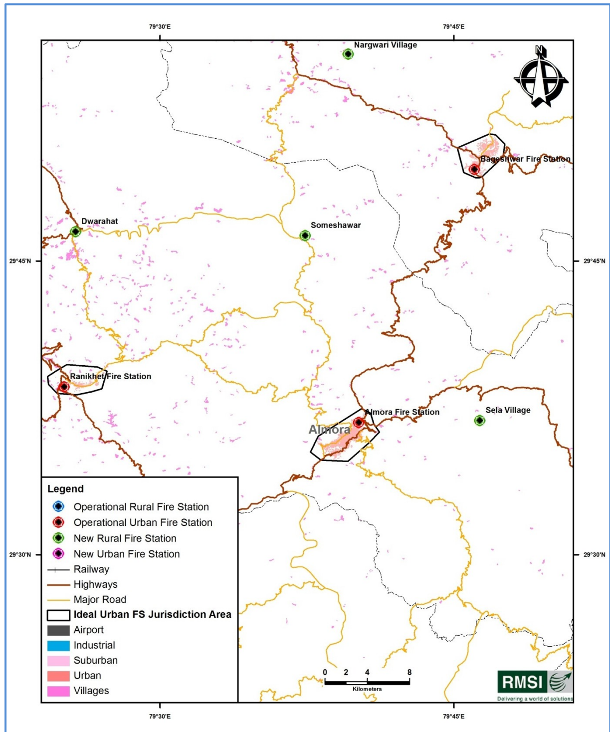
Figure 17-14: Fire Stations gap analysis for Almora urban areas
