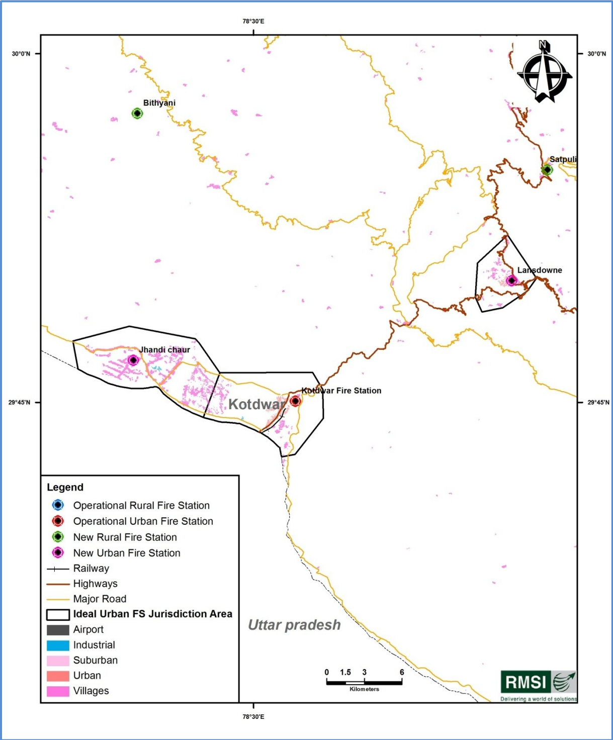
Figure 17-16: Fire Stations gap analysis for Kotdwar urban areas
