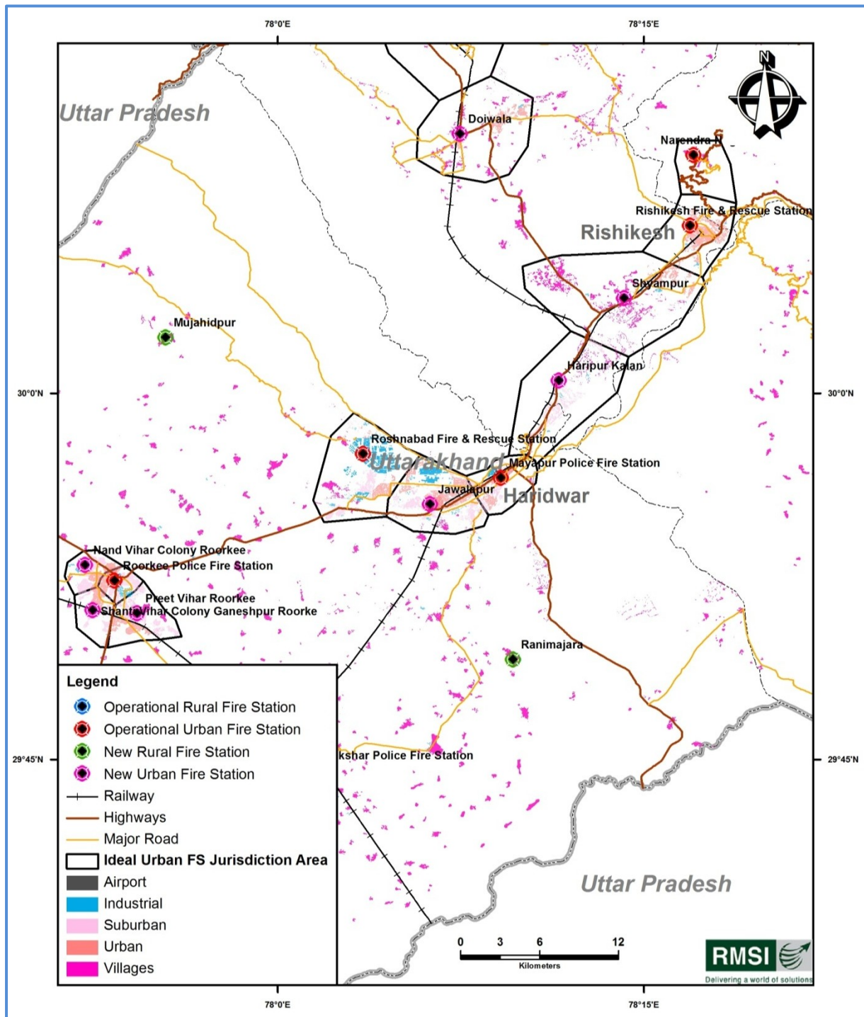
Figure 17-7: Fire Stations gap analysis for Hardwar and Rishikesh rural areas
