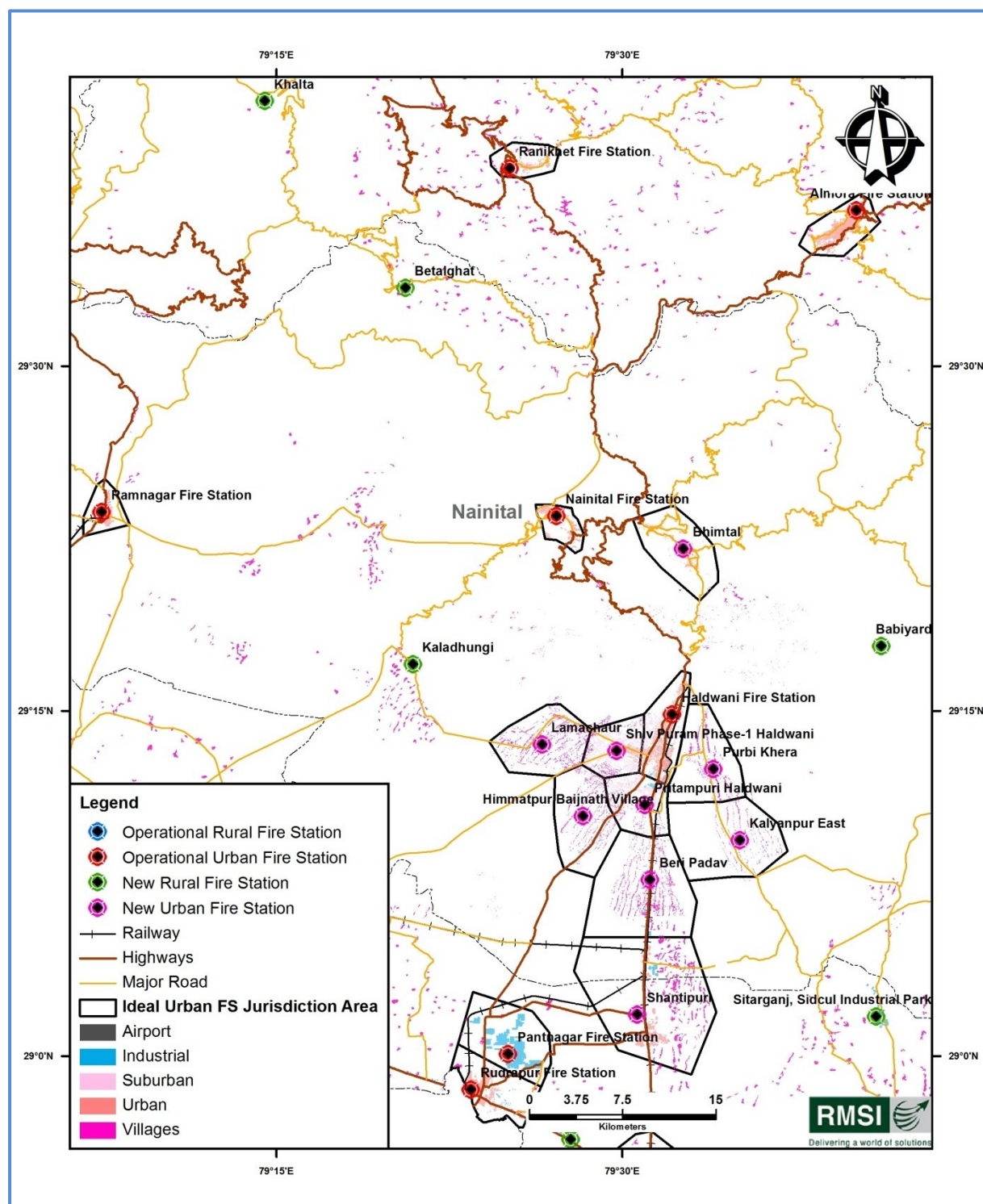
Figure 17-13: Fire Stations gap analysis for Nainital rural areas
